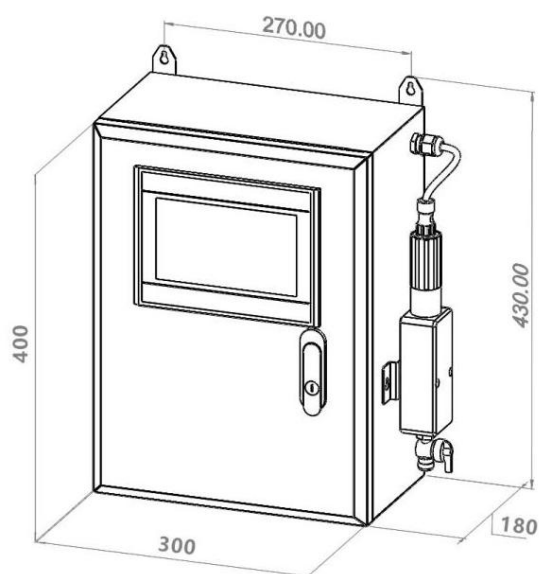
Fig.1 Protective box dimensions
