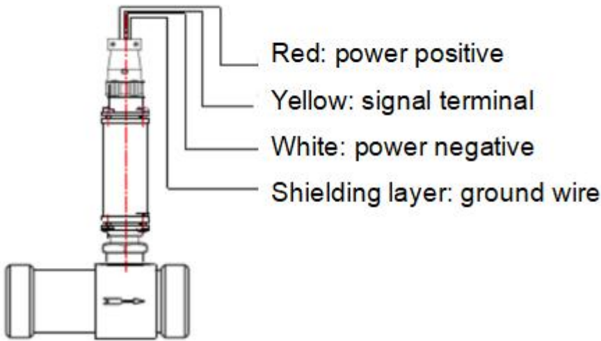
Figure1 Figure 11 Wiring diagram of sensor and display instrument
